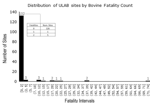
Fig. 5 Approximately 86.3% (126/146) of sites are responsible for zero fatalities, 6.2% (9/146) of sites induce minor damages (1 to 5 fatalities), 4.1% (6/146) induce moderate damages (6 to 20 fatalities), and 3.4% (5/146) induce severe damages (21+ fatalities)
