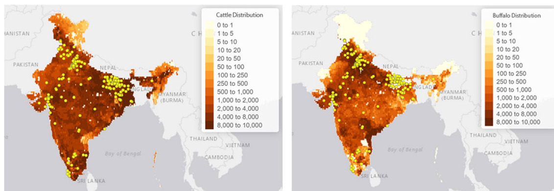
Fig. 2 FAO gridded bovine densities for India overlaid with the 146 lead contaminated sites used in the analysis
