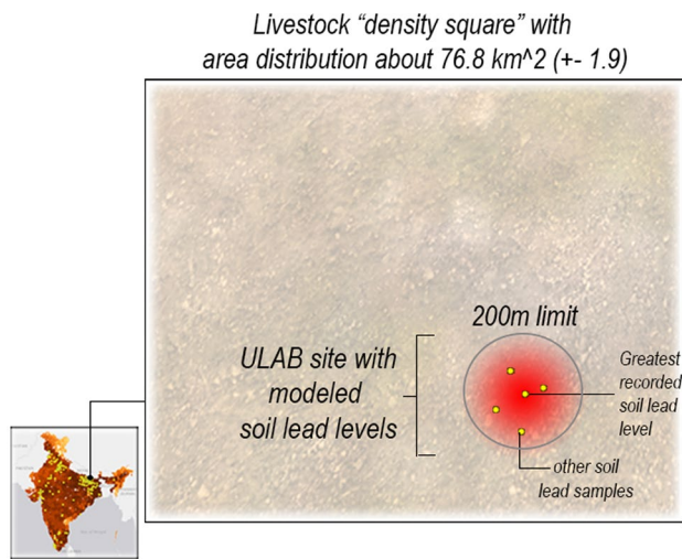
Fig. 3 Depiction of a ULAB site modeled within an FAO livestock density square. We estimated the site's total soil lead contamination with a linear model based on a Poisson plume diffusion equation (Eq. 1) using the highest measured soil lead level as the center of the site. The proportion of contaminated land to the area of the livestock density square is assumed to equal the portion of livestock potentially exposed to soil lead
