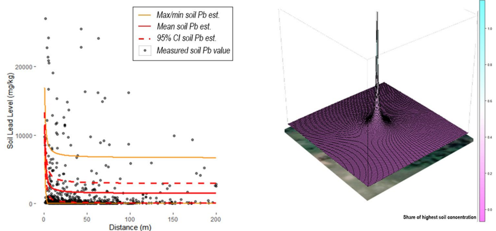
Fig. 4 Left: the actual soil lead level data with the linear OLS regression outcomes, with min, max, and 95% CI, at each site in one dimension. Right: an example of a three-dimension projection of the soil modeling outcome at a given site. Both the height of the curve and the color represent the relative soil lead values emanating out from the highest recorded soil lead point
